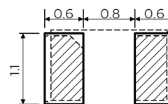
Top View Suggested Layout
