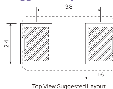
Top View Suggested Layout
