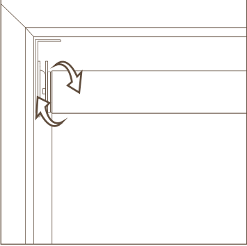
3 Align the bracket with the mounting hole and rotate clockwise
