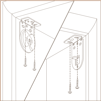
3 Tighten the screws to fix the bracket
