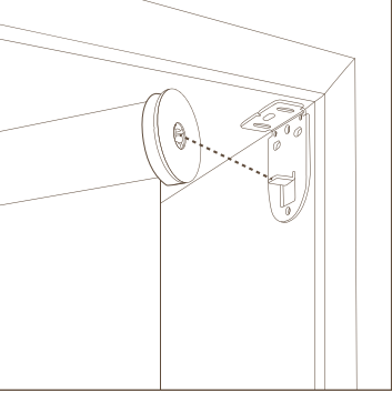
1 Align the connector and install it into the bracket
